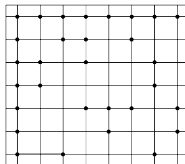
Figure 5: First step of canceling A_6 from the family F in Example 1. We marked a horizontal section in the 6-th row.
