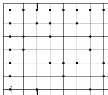
Figure 6: We linked out the row of A_6 and marked a vertical section.
