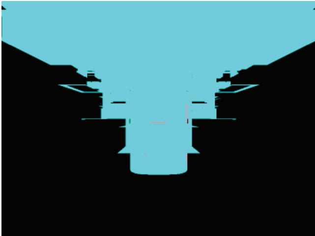
Figure 5 - Result of the visibility detection algorithm using view window coupled with a larger visibility surface. There are a few false negatives and a few false positives, which we do not see here, since the size of the view window is constant.
