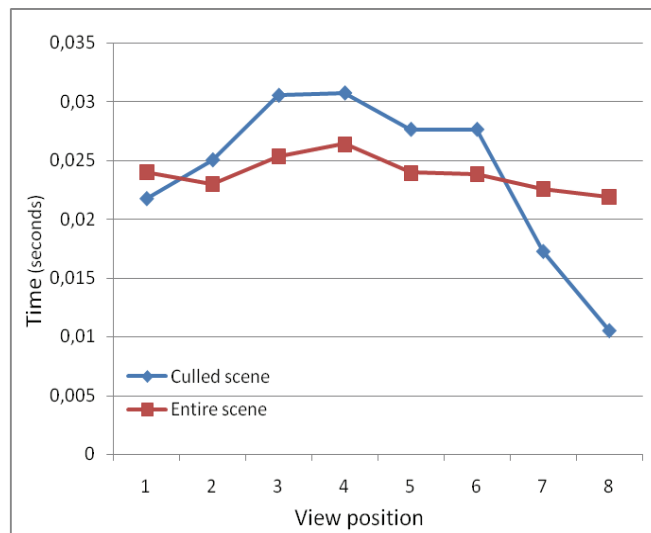
Figure 1 - Comparison of the performance of the algorithm with and without usage of culling.
