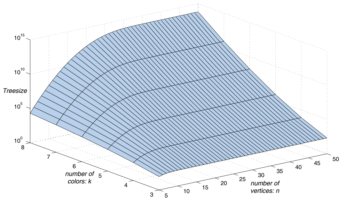
Figure 3: Expected size of the search tree for p = 0.5 , as a function of n and k .
