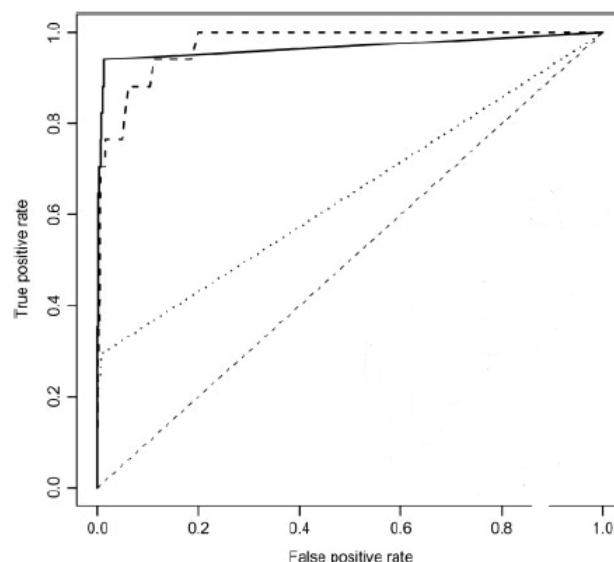
Figure 1: ROC curve
