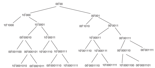
Figure 2: Code words derived from 00^i0 when i is even
