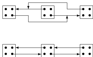
Figure 2: Bottom: A horizontal portion of the double linked list. Top: The middle entry is linked out horizontally.
